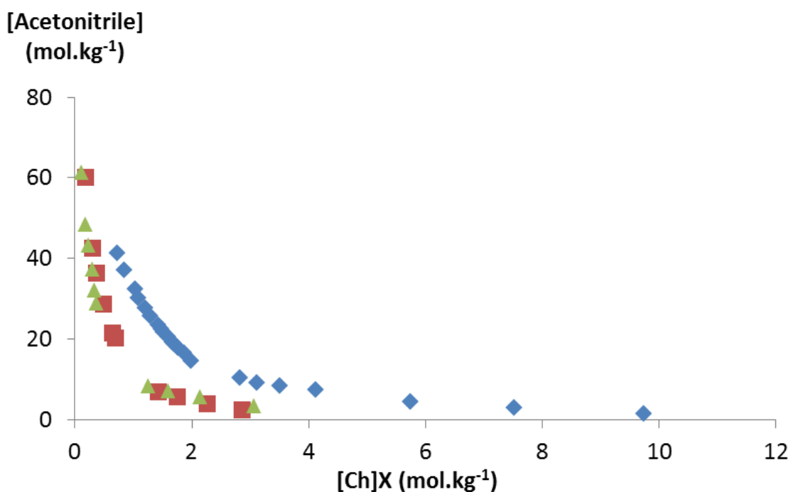
Figure 1: Phase diagrams for the ternary systems composed of acetonitrile + [\text{Ch}]\text{X} + water at 25°C: ( \diamond ) [\text{Ch}]\text{Cl} , ( \blacksquare ) [\text{Ch}][\text{Bit}] , and ( \blacktriangle ) [\text{Ch}][\text{DHCit}] .
