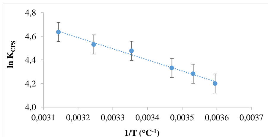
Figure A3: Relationship between K_{CPS} - \ln(K_{CPS}) - versus T^{-1} ( ^{\circ}C^{-1} ) for the CPS partitioning considering the system 20 wt% of acetonitrile + 15 wt.% of K_2CO_3 + 65 wt.% water at different temperatures.
