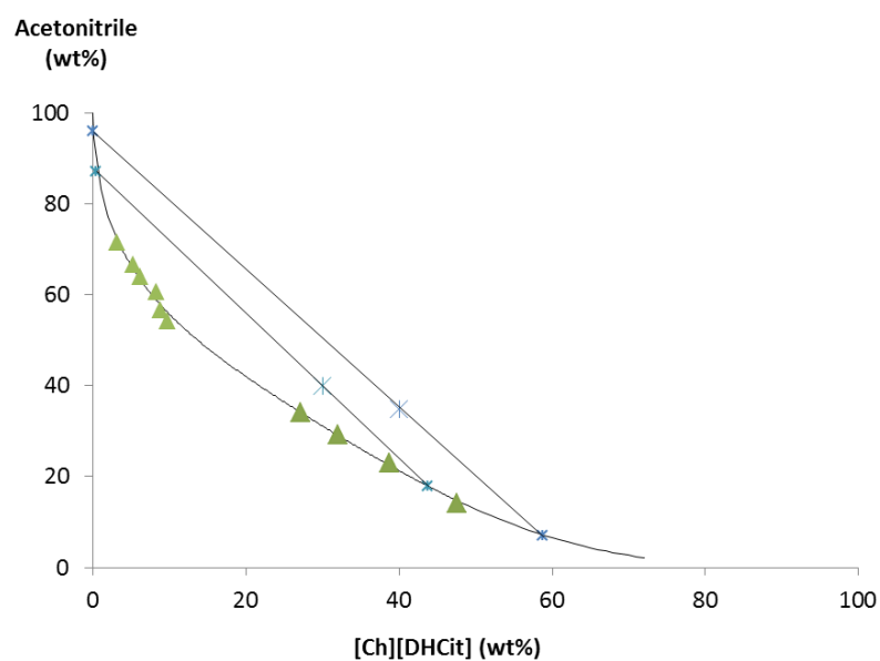
Figure A2: Phase diagrams for the ternary systems composed of acetonitrile + [Ch]X + water at 25°C. (♦) [Ch]Cl, (■) [Ch][Bit], (▲) [Ch][DHCit], (*) tie-line data, (—) binodal curve adjusted data through Eq. (1).
