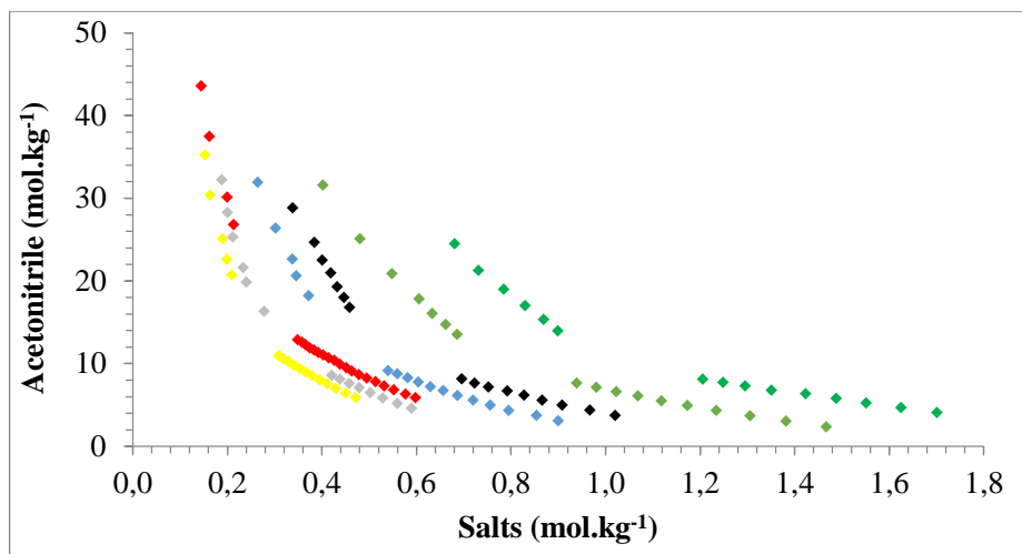
Figure 1: Phase diagrams to the ternary system composed of acetonitrile + salt + water at 25°C. (♦) C_6H_5K_3O_7 , (♦) C_6H_5Na_3O_7 , (♦) Na_2S_2O_3 , (♦) K_3PO_4 , (♦) K_2HPO_4 , (♦) K_2CO_3 , (♦) Na_2CO_3 .
