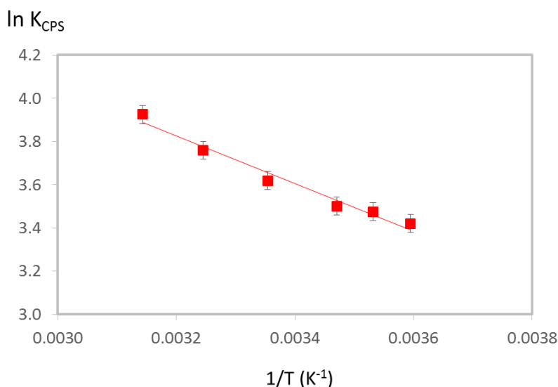
Figure 3: Correlation between the logarithmic function of K_{CPS} - \ln(K_{CPS}) - versus T^{-1} ( \text{K}^{-1} ) for the CPS partitioning considering the system 30 wt% of acetonitrile + 35 wt% of [Ch]Cl + water at different temperatures, namely 318, 308, 298, 288, 283, 278 ( \pm 1 ) K.
