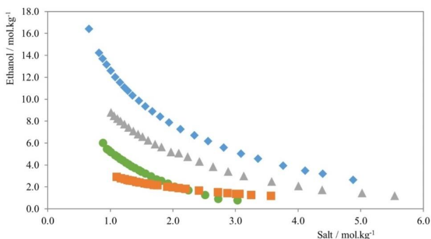
Figure 2. Binodal curves for ternary systems composed of ethanol + salt + water at 298 K and atmospheric pressure. ( \blacklozenge ) [\text{Na}_2\text{S}_2\text{O}_3] ; ( \blacktriangle ) [\text{NaH}_2\text{PO}_4] ; ( \bullet ) [\text{Na}_2\text{CO}_3] , ( \blacksquare ) [\text{Na}_2\text{SO}_4] .
